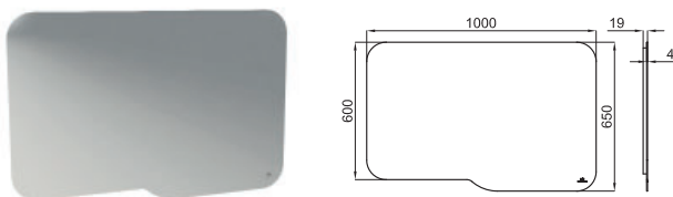
FORMA. Horizontal mirror with smooth and rounded edges, 100x65 cm Miroir horizontal de 100x65 cm. à bords polis.
