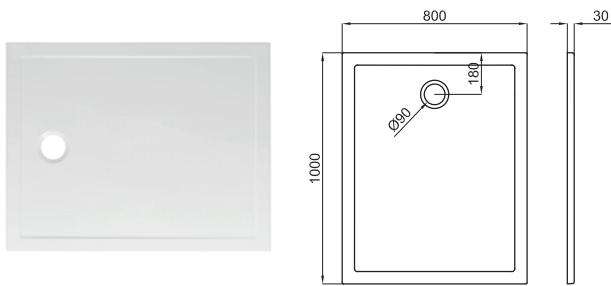
100x80 ceramic shower tray Receveur de douche 100x80 ceramique
