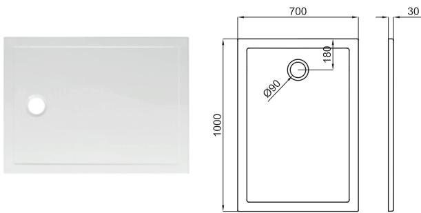
100x70 ceramic shower tray Receveur de douche 100x70 ceramique
