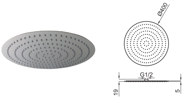
Rondo 40 cm. rain shower head, without ball joint. Flow rate 12 l/min. at 3 bar. Pomme de douche Rondo 40 cm, sans articulation. À 3 bars de pression
